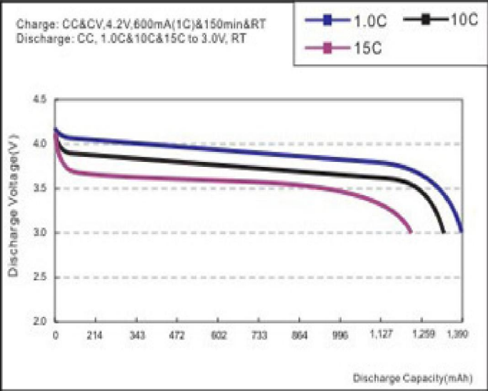
Discharge rate characteristics
