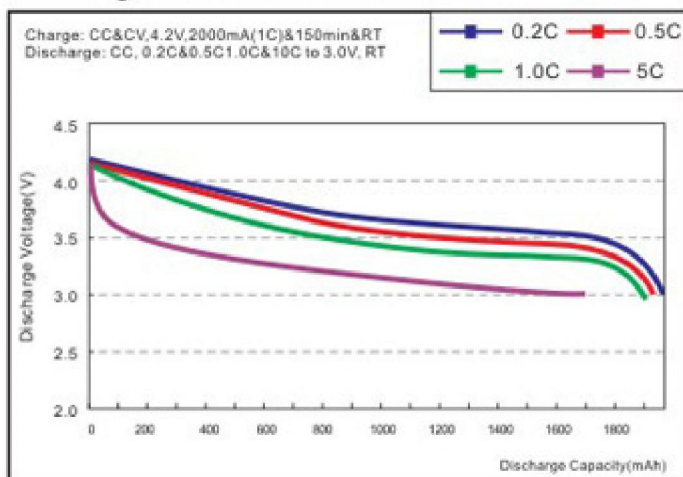
Discharge rate characteristics
