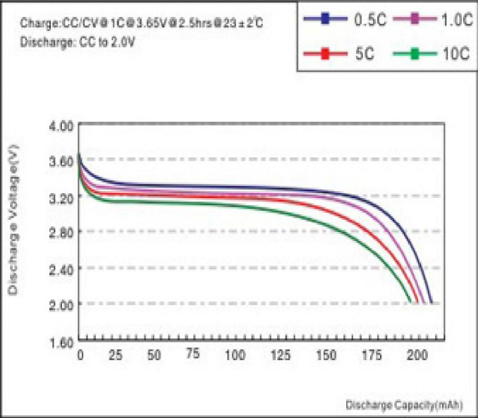
Discharge rate characteristics
