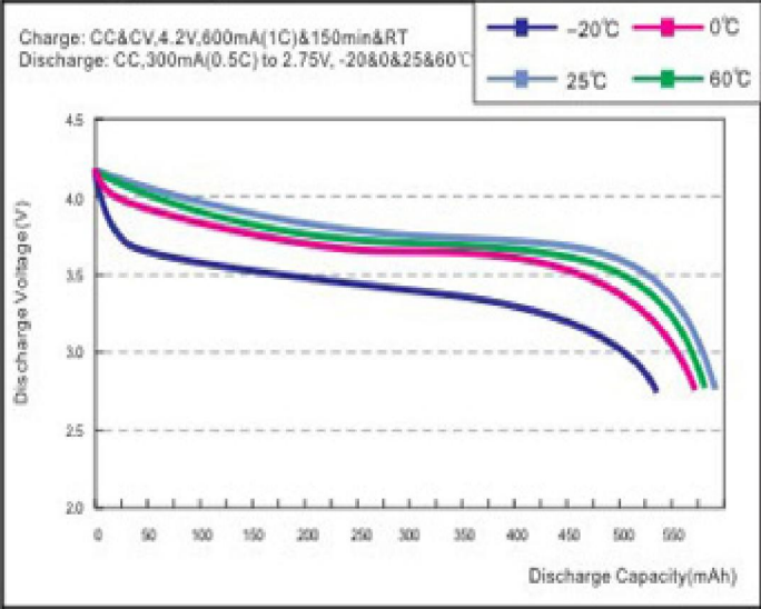
Discharge temperature characteristics
