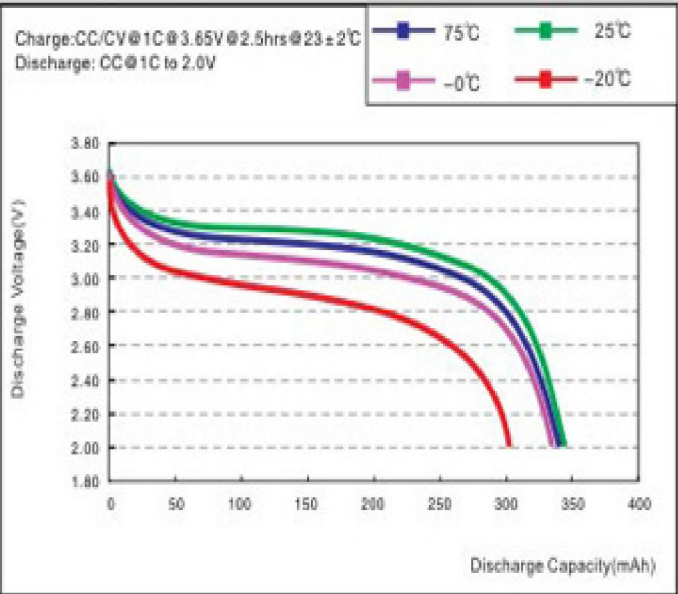
Discharge temperature characteristics
