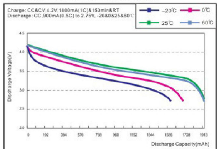
Discharge temperature characteristics
