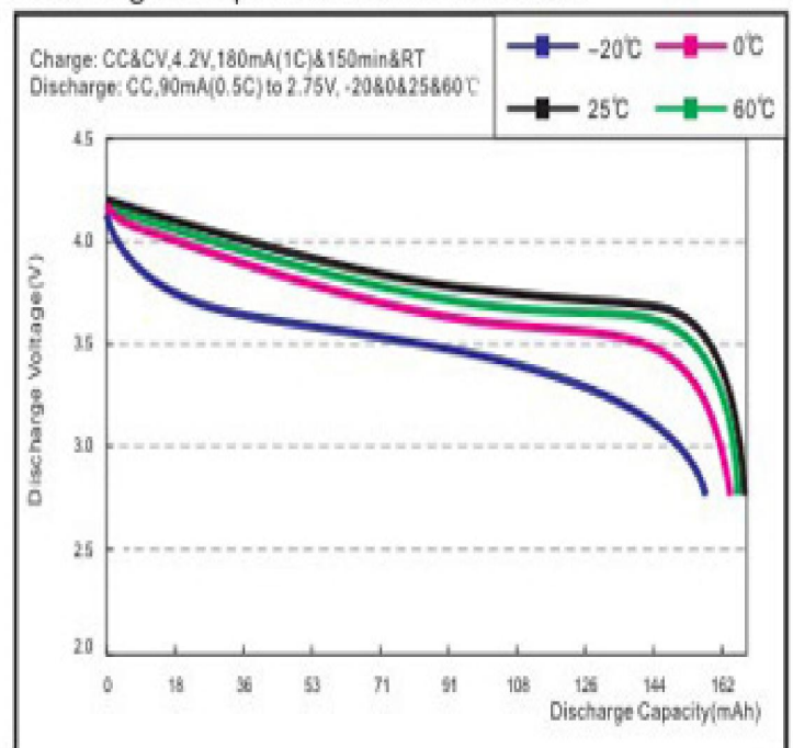
Discharge temperature characteristics
