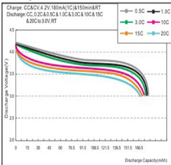
Discharge rate characteristics
